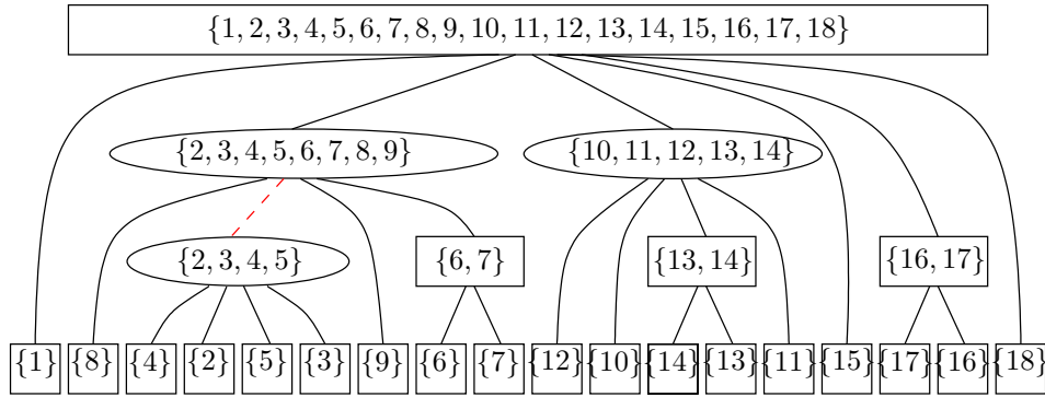
Figure 1: The strong interval tree T_S(\sigma) of the permutation \sigma = (1 \bar{8} 4 2 \bar{5} 3 9 \bar{6} 7 12 10 \bar{14} 13 \bar{11} 15 17 16 18) . Prime and linear vertices are distinguished by their shape. There are three non-trivial linear vertices, the rectangular vertices, and three prime vertices, the round vertices. The root and the vertex \{6, 7\} are increasing linear vertices, while the linear vertices \{16, 17\} and \{13, 14\} are decreasing.
