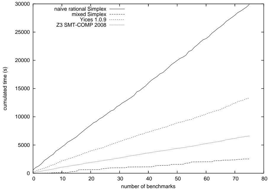
Fig. 2. Benchmarks on systems of 100 inequalities with 50 variables, where all coefficients are taken uniformly and independently distributed integers in [-100, 100] . 31 are unsatisfiable, 46 are satisfiable.
