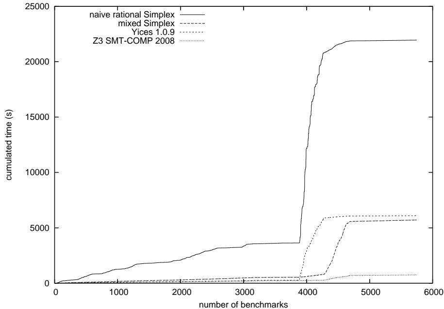
Fig. 1. Benchmarks on unsatisfiable conjunctions extracted from verification SMT problems. Even though our implementation of sparse arithmetic and the rational simplex are not up to those in state-of-the-art solvers (as shown by the lack of performance on the “easy” examples on the left), and our procedure is not geared towards the sparse problems typical of verification applications, it still performs faster than Yices 1.
