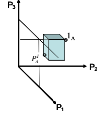
Figure 1: The upper hypercube P_A^I - 1_A lower bound P_A^I - upper bound 1_A
