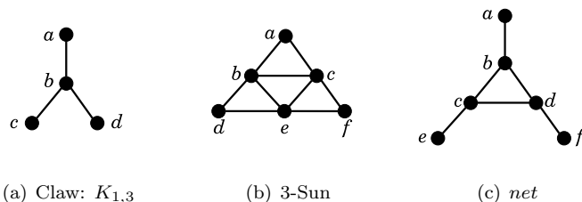
FIGURE 3. Forbidden induced subgraphs for proper interval graphs.
