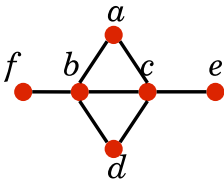
FIGURE 2. An exemple of graph on which MCS , LexBFS fail to find a max-min simplicial vertex. For any starting vertex, both searches will end on e or f .
