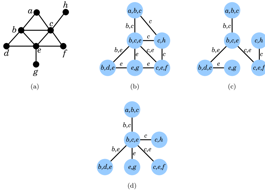
FIGURE 1. An example of a chordal graph (a), its reduced clique-graph (b), note that although the maximal cliques \{b, d, e\} and \{c, e, f\} intersect the corresponding edge is missing. Two maximal clique-trees are shown (c)-(d).
