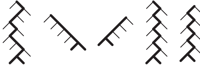
FIGURE 1. Thin trees, with their spines in bold: from left to right, \langle 1001011100 \rangle , which is also \langle 100101101 \rangle , the right comb of size 5, the left comb of size 4, the right zigzag of size 9, the left zigzag of size 8.
