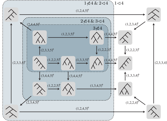
FIGURE 10. Names of edges and covering relation in the associahedron K_4 . The regions correspond to the various possibilities for covering by 4. As i < 4 implies j < 4 for i < j < 4 , there are four regions corresponding to 1 < 4 , to 1 \not< 4 and 2 < 4 , to 2 \not< 4 and 3 < 4 , and to 3 \not< 4 . Lemma 3.13 says for instance that the only way to leave the region 3 \not< 4 is to cross a pair named (\dots, 4, 4, \dots)^+ .
