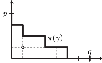
FIGURE 6. Application of Lemma 2.22 to \gamma = 101001001 with p = 4 and q = 7 : we find p - \#_1\gamma = 4 - 4 = 0 , q - \#_0\gamma = 7 - 5 = 2 , the number of squares below \pi(\gamma) touching one of the axes is 7, and the distance from (1, 1) to the region above \pi(\gamma) is 1, leading to f(4, 7, \gamma) = 0 + 2 + 7 + 1 = 10 . Hence, if T and T' are trees in which, for some i , the i th leaf has address 1^4 0^7 in T and \gamma in T' , we have \text{dist}(T, T') \geq 10 .
