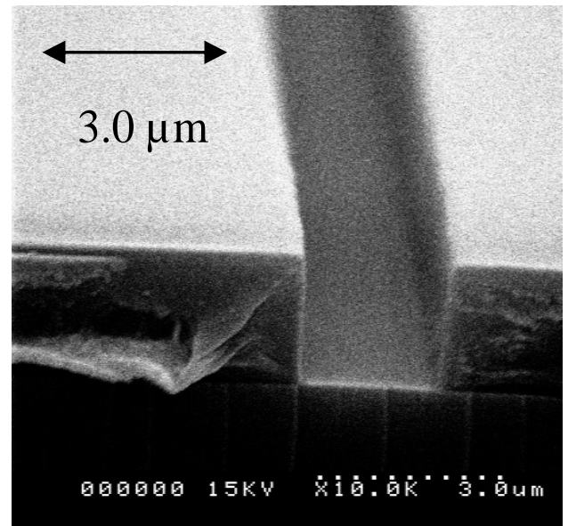
Fig. (13). SEM photo of PMMI hollow waveguide 2.5 \times 2.5 \mu m^2 .
