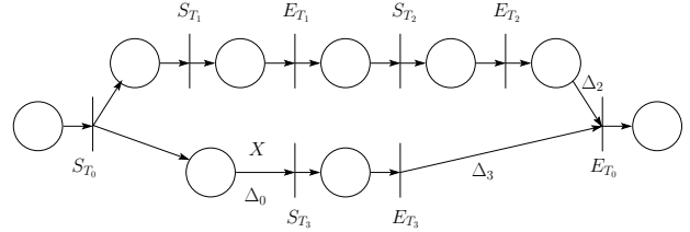
(b) The associated Petri net
