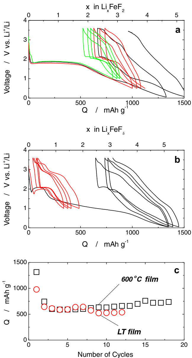
Fig. 4. Discharge and charge curves of lithium cells using iron fluoride thin films as positive electrode. Films were deposited on stainless steel substrates from FeF 3 target under vacuum of 5.0 \times 10^{-5} Pa at several substrate temperatures, i.e., 600 (a) and -50 °C (b). The cells were tested in various voltage windows 3.6 to 1.0, 0.5 and 0.05 V at a current density of 1 \mu\text{A}/1.77 \text{ cm}^2 ( 0.56 \mu\text{A} \cdot \text{cm}^{-2} ) (a,b), and 5 \mu\text{A}/1.77 \text{ cm}^2 ( 2.8 \mu\text{A} \cdot \text{cm}^{-2} ) (c) at 25 °C. The electrolyte used was 1 M LiPF 6 dissolved in EC / DMC solution (1/1 by volume). (c) Corresponding capacity versus the number of cycles curves.
