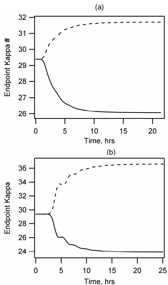
Fig. 9. Symmetric step tests for (a) \pm 0.15 \text{ m}^3/\text{min} change in dilute liquor flow; and (b) \pm 0.15 \text{ m}^3/\text{min} change in white liquor flow
