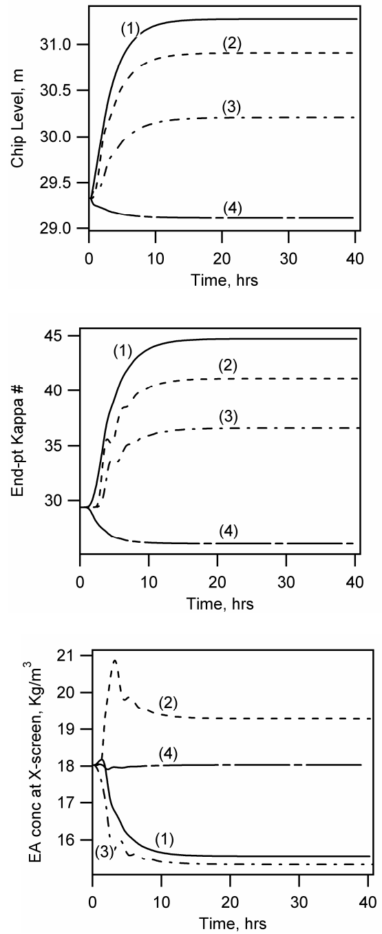
Fig. 7. Dynamic behavior for (1) increase in blowline flow; (2) decrease in upper heater temp.; (3) decrease in white liquor; and (4) decrease in dilute liquor flow.
