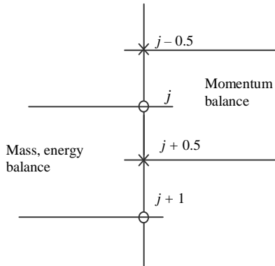
Fig. 3. Arrangement of overlapping control volumes on digester vessel
