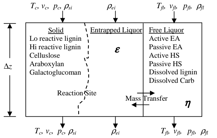
Fig. 2. A cross-sectional slice of digester consists of solid, entrapped liquor and free liquor phases.
