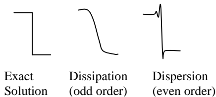
Fig. 4. Use of finite differences induce numerical diffusion
