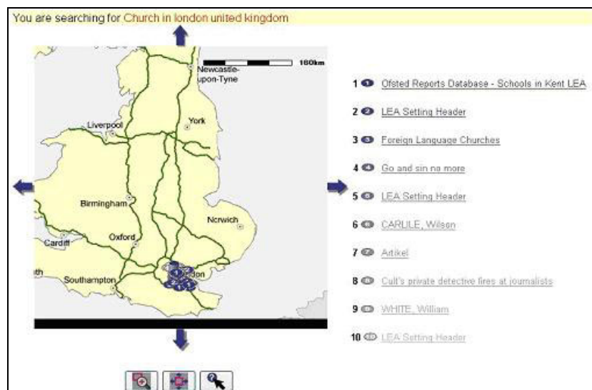
Figure 8: SPIRIT screenshot
