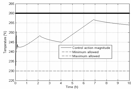
Figure 2. Constrained control temperature tuned by the MPC@CB software during the primary stage.
