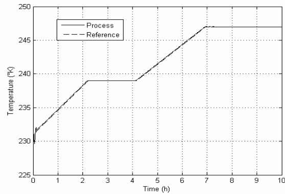
Figure 1. Temperature trajectory tracking results during the primary stage.
