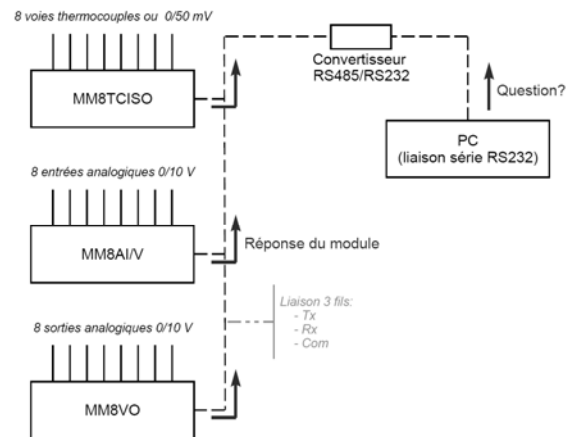
Figure 4 : Système acquisition-commande
