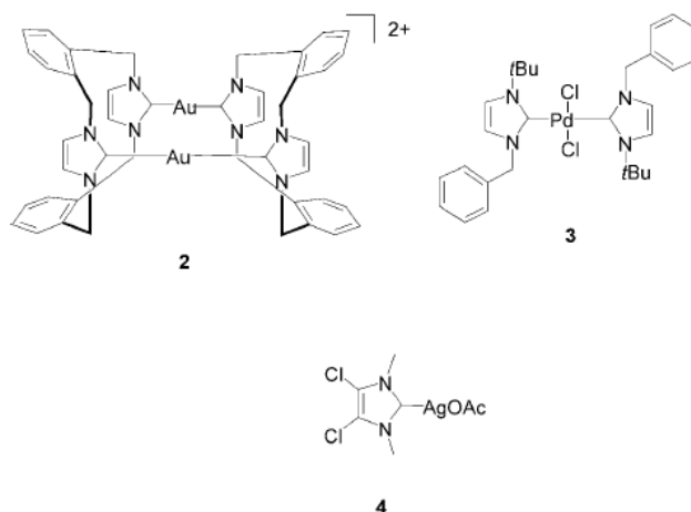
Scheme 1. Metal–NHC complexes reported for their anti-proliferative properties.
