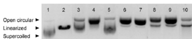
Figure 6. Effect of additives on DNA cleavage. Line 1: supercoiled plasmid; line 2: plasmid linearized by using the endonuclease BamHI; line 3: [CuCl(SiMes)] (5), 3 h; line 4: 5, 24 h; line 5: 5 + NaNO 3 , 24 h; line 6: 5 + ascorbic acid, 3 h; line 7: 5 + GSH, 3 h; line 8: Cu(phen) 2+ + GSH, 3 h; line 9: 5 + GSH, 24 h; line 10: 5 + GSH, 48 h. Concentration of all complexes: 10 μM; supercoiled plasmid: 1.6 μg.
