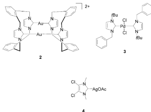
Scheme 1. Metal–NHC complexes reported for their anti-proliferative properties.
