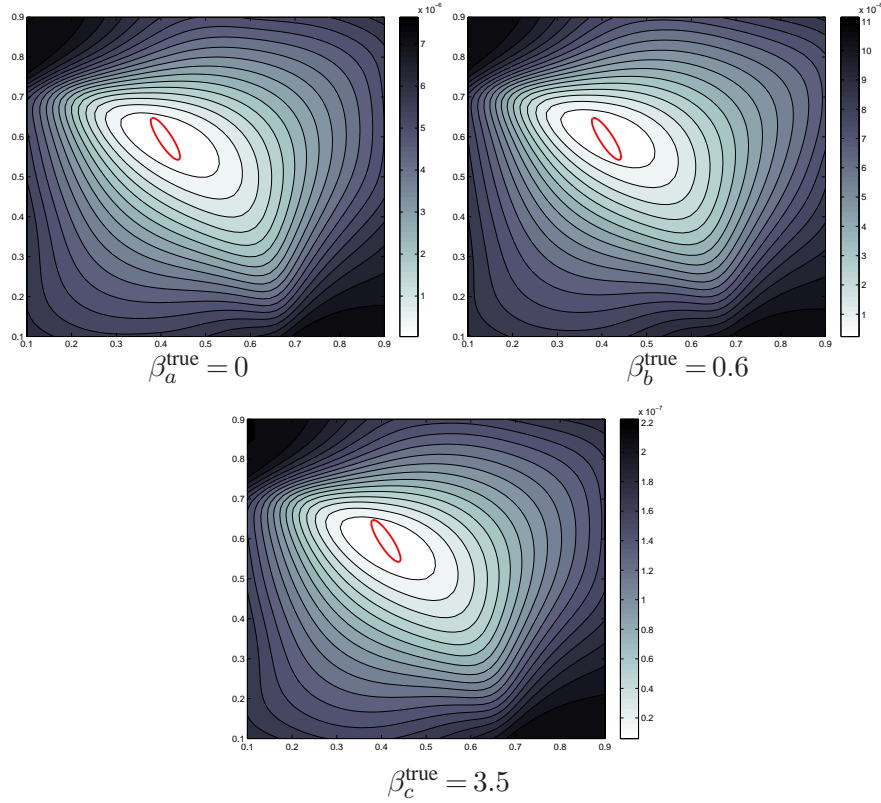
Figure 10: Identification of inclusion 3 (elliptical): distribution of J^{\min} over search grid \mathbf{G} , and outline of true inclusion (noisy data, with 20% noise on u^{\text{obs}} - u ).
