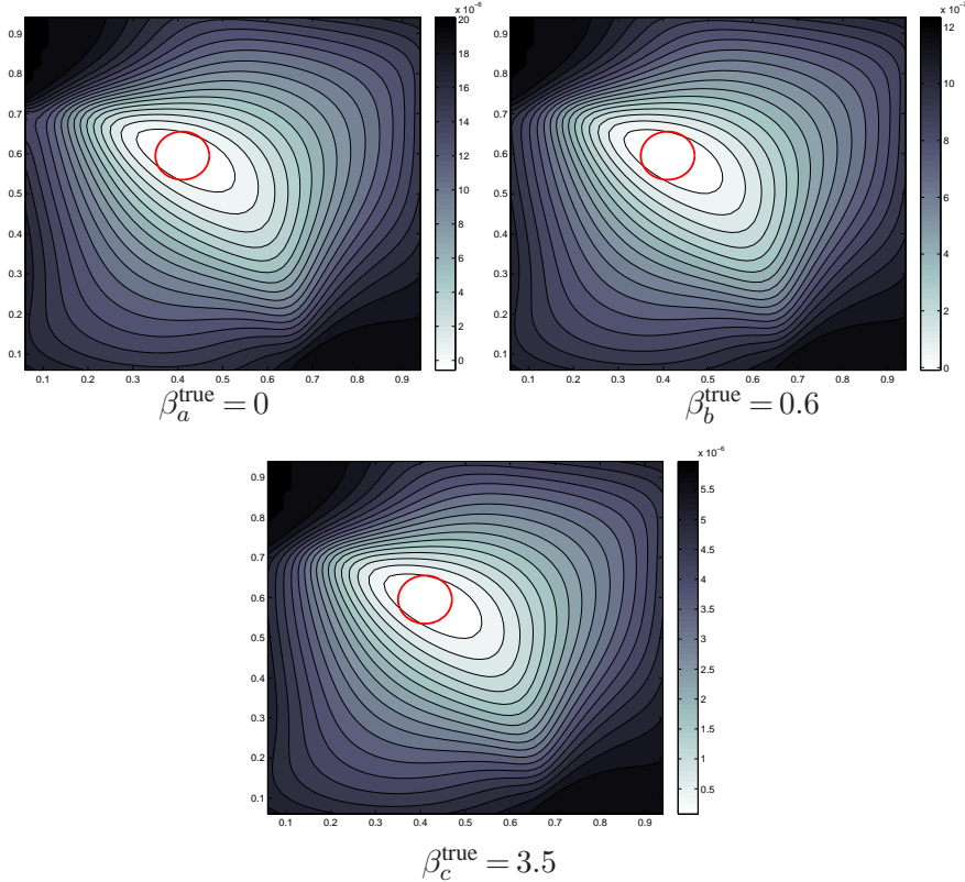
Figure 7: Identification of inclusion 1 (circular): distribution of J^{\text{min}} over search grid \mathbf{G} , and outline of true inclusion.
