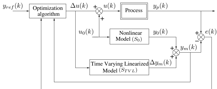
Fig. 3. General Linearized IMC-MPC structure.
