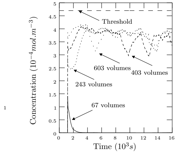
Fig. 9. Run #2: Mean concentration of pollutant at the process outlet for various finite dimension approximations of (S_{TVL}) .
