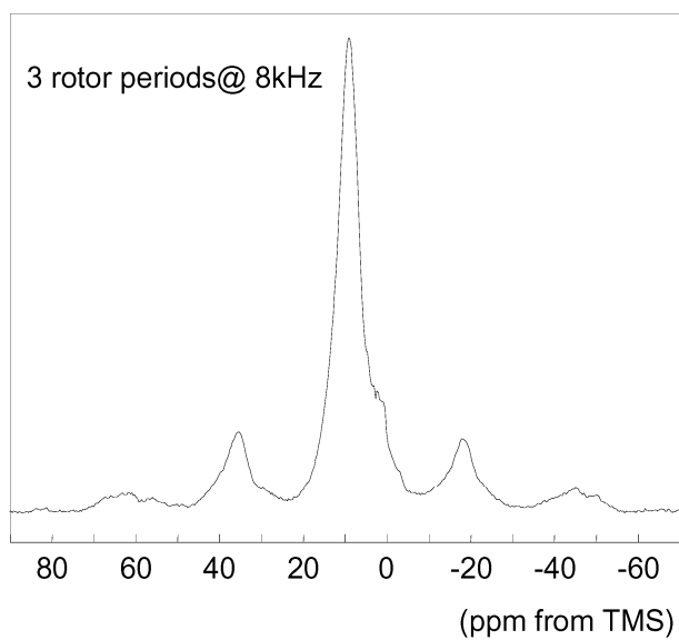
Figure 6. ^1H MAS NMR spectrum of raw-sample
