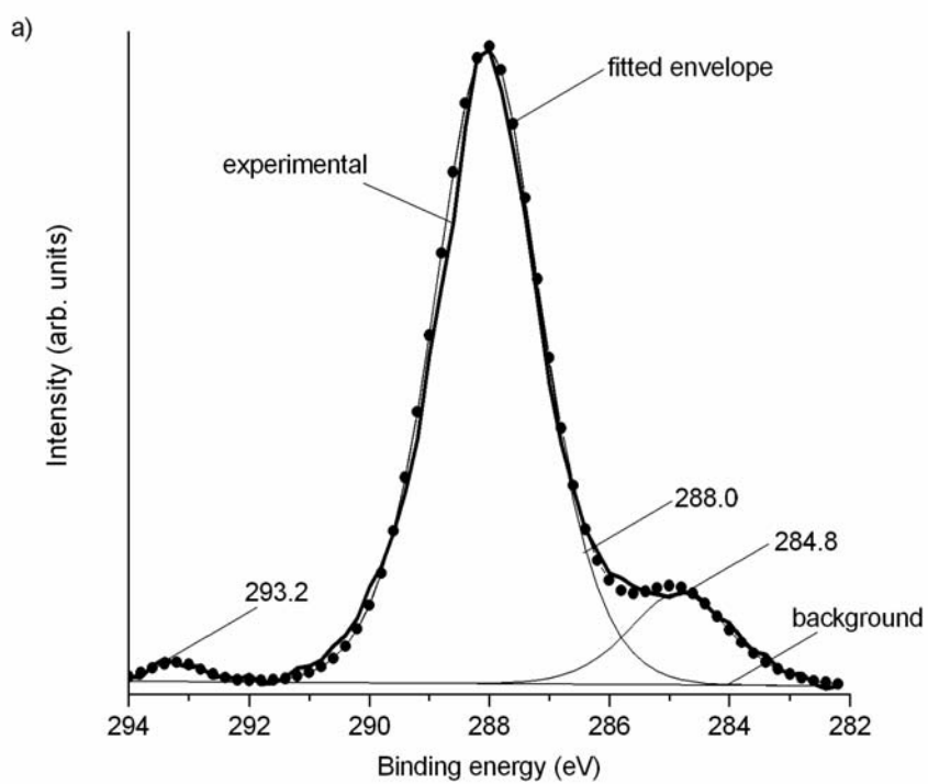
Figure 4. Experimental and fitted XPS spectra of raw-sample a) C1s and b) N 1s
