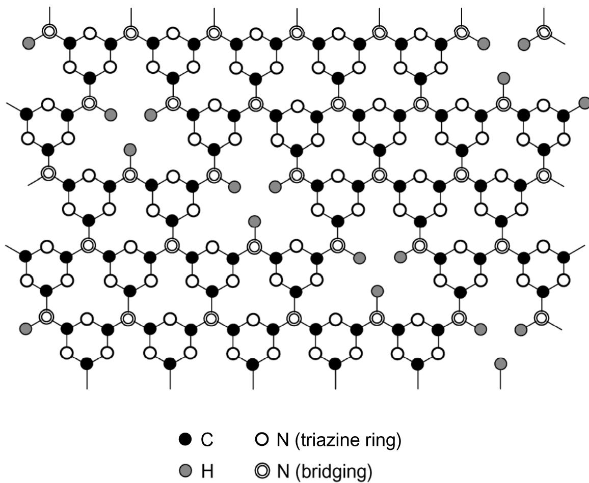
Figure 7. Schematic representation of C_3N_{4.2}H_{0.6} framework with an ordering of voids in a Triazine model
