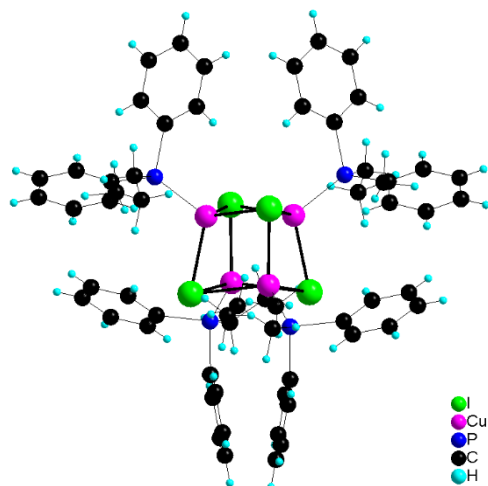
Figure 3. Molecular structure of C2 [ \text{Cu}_4\text{I}_4(\text{PPh}_2(\text{CH}_2)_2\text{CH}_3)_4 ].
