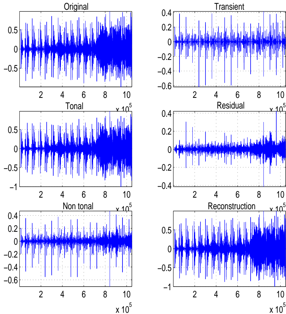
FIGURE 10. Compressed hybrid expansion of a piece of music (mamavatu, about 6 seconds long.) From top to bottom, and from left to right: original signal, tonal layer, nontonal signal, transient layer, residual layer, and reconstruction from the three layers.
