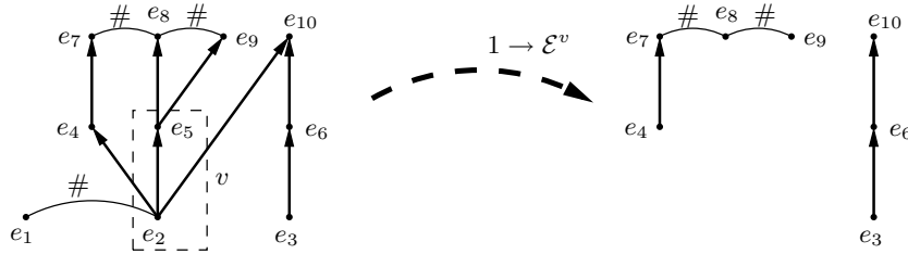
Figure 3: An event structure \mathcal{E} and a configuration v of \mathcal{E} . The future of v = \{e_2, e_5\} is shown on the right.
