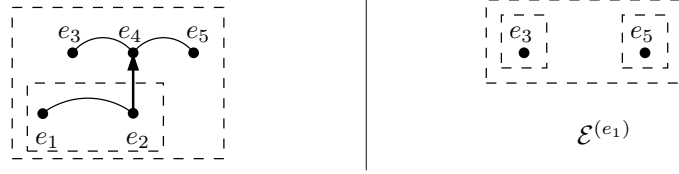
Figure 7: Left, an event structure \mathcal{E} . Right, the future of configuration (e_1) . All nonempty stopping prefixes are depicted by dashed frames. The concatenation of two stopped configurations is not stopped: (e_1 e_3) is the concatenation of two stopped configurations, but (e_1 e_3) is not stopped in \mathcal{E} .
