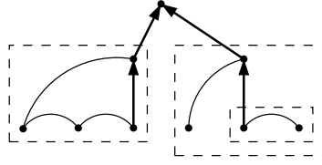
Figure 4: An event structure with minimal conflicts depicted by curved arcs. Some stopping prefixes are depicted by dashed frames.
