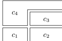
Figure 9: Showing the collection of branching cells \Delta(\omega) , for \omega as in Figure 8.
