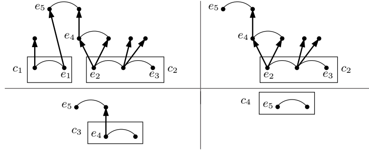
Figure 8: Decomposition of \omega = (e_1e_2e_3e_4e_5) through branching cells to determine \Delta(\omega) . The possible choices of branching cells at each step are depicted by rectangles.
