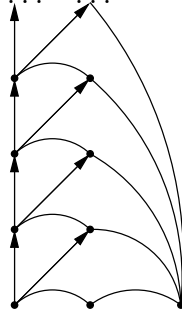
Figure 6: An event structure uniformly pre-regular, but non locally finite: the event at right-bottom is in immediate conflict with infinitely many events.
