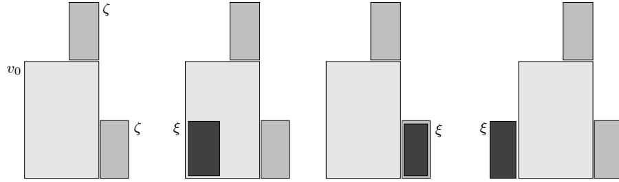
Figure 10: Illustrating Lemma A.5. The first diagram shows v_0 \oplus \zeta , with two possible positions for \zeta . The other diagrams show the possible situations for \xi , corresponding to “first case”, “second case (a)”, and “second case (b)” of the proof, which yield \zeta' = \zeta , \zeta' = \emptyset , and \zeta' = \zeta , respectively.
