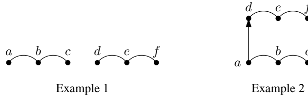
Figure 1: Two event structures. Curved lines denote conflict and directed arrows denote causality.
