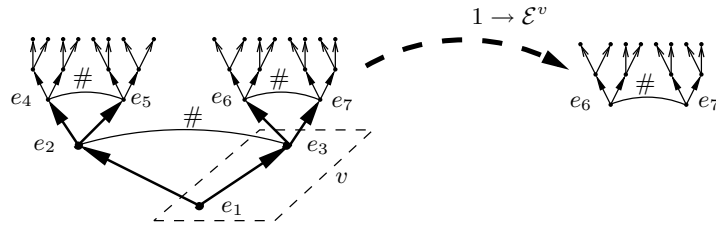
Figure 2: Left, a tree of events. Immediate successors of a same events are pairwise in conflict. The future of v = \{e_1, e_3\} is depicted on the right.
