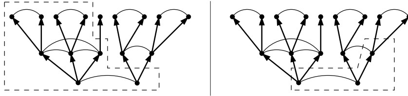
Figure 5: Left: a stopping prefix of a tree of events. Right: a prefix which is not a stopping prefix.
