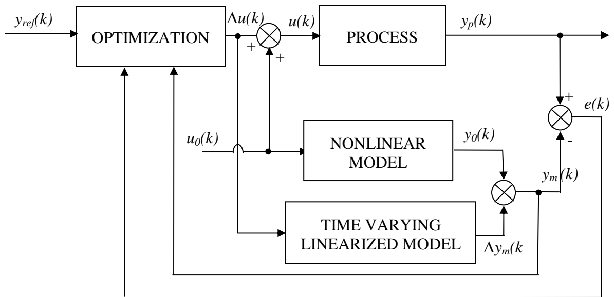
Fig. 1: General MPC structure used.
