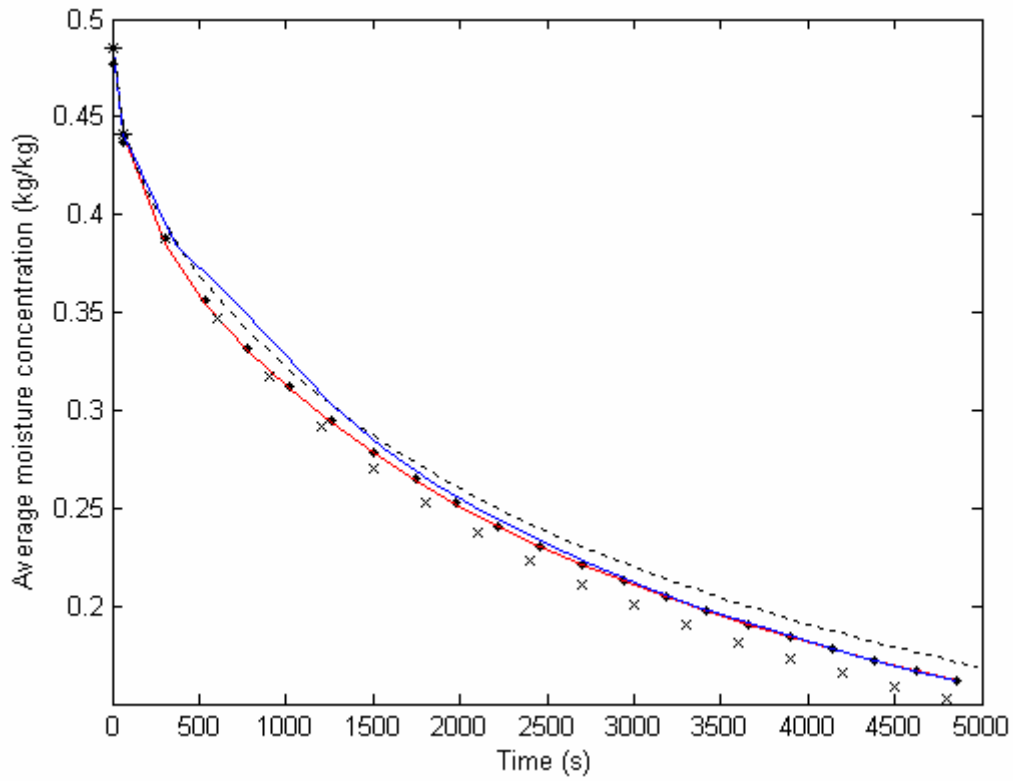
Fig. 2: Reference trajectory tracking: reference curve (•••) for the drying process output: with open loop control while u=u_0=[49.5^\circ\text{C } 10.0\%] (x) and u=u_0=[45.0^\circ\text{C } 20.0\%] (- - -), with the MISO PID (—) and with the MISO MPC (—) with a 5 point horizon prediction, each case with uncertainties: 1.68% error on the initial moisture concentration and 10.0% error on the diffusion coefficient.
