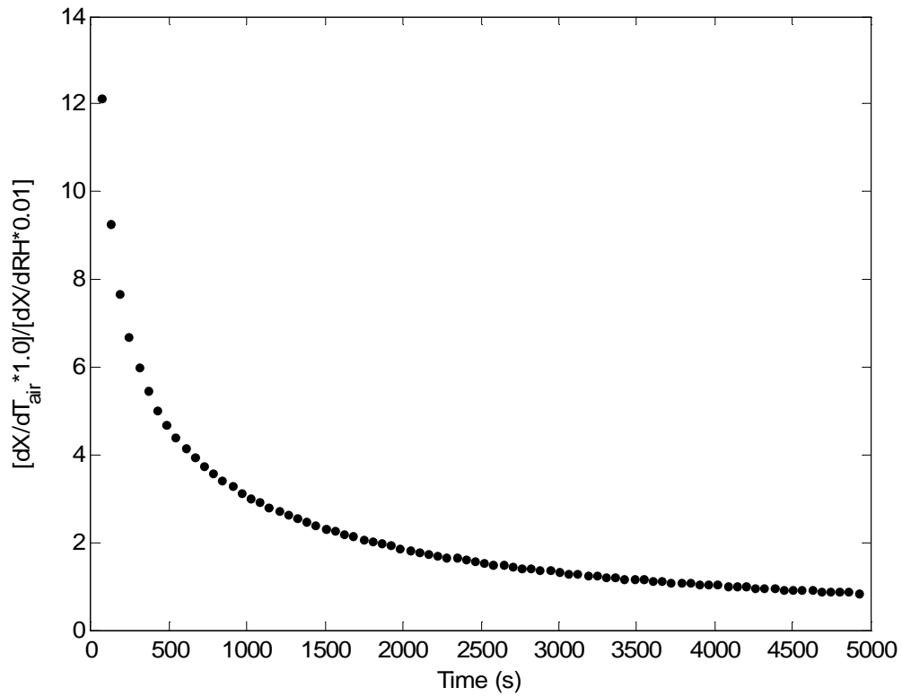
Fig. 5: The ratio between the sensitivities of the air temperature and mean relative humidity with respect to an air temperature input of 1.0°C and with respect to a relative humidity input of 1.0%, measured for the drying process at 49.5°C and 10.0%.
