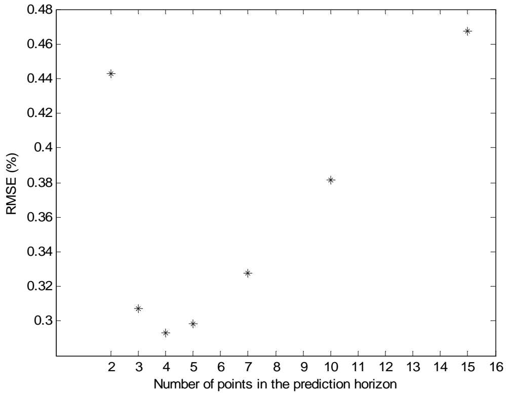
Fig. 6: The impact of the tuning of the prediction horizon of the MPC on the RMSE, each case with uncertainties: 1.68% error on the initial moisture concentration and 10.0% error on the diffusion coefficient.
