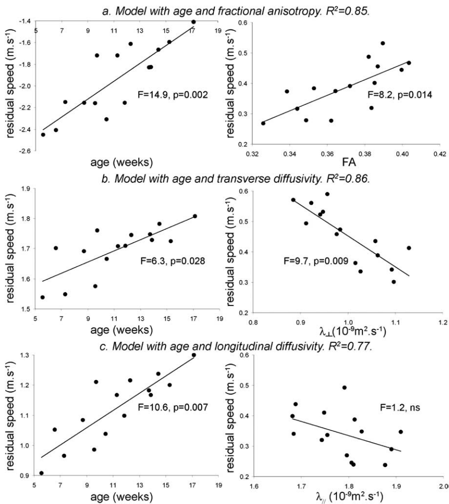
Figure 2. Changes in conduction speed across the infant group with age and DTI indices in the optic radiations. a–c , For the models detailed in Table 1, with age and DTI index covariates (FA, \lambda_{\perp} , \lambda_{//} ), the plots represent the variations of residual speed, as a function of age after correction for the DTI index effect (left column, speed – \beta DTI index) and as a function of DTI index after correction for the age effect (right column, speed – \alpha age). The contribution of the DTI index was significant for FA and \lambda_{\perp} , but not for \lambda_{//} . ns, Not significant.
