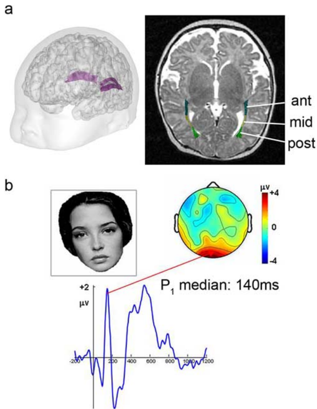
Figure 1. a , Reconstruction by tractography of the optic radiations, with three segments. b , Visual evoked response to faces: grand-average across all infants measured across six electrodes around Oz, and P 1 topographic map at 140 ms. ant, Anterior; mid, middle; post, posterior.
