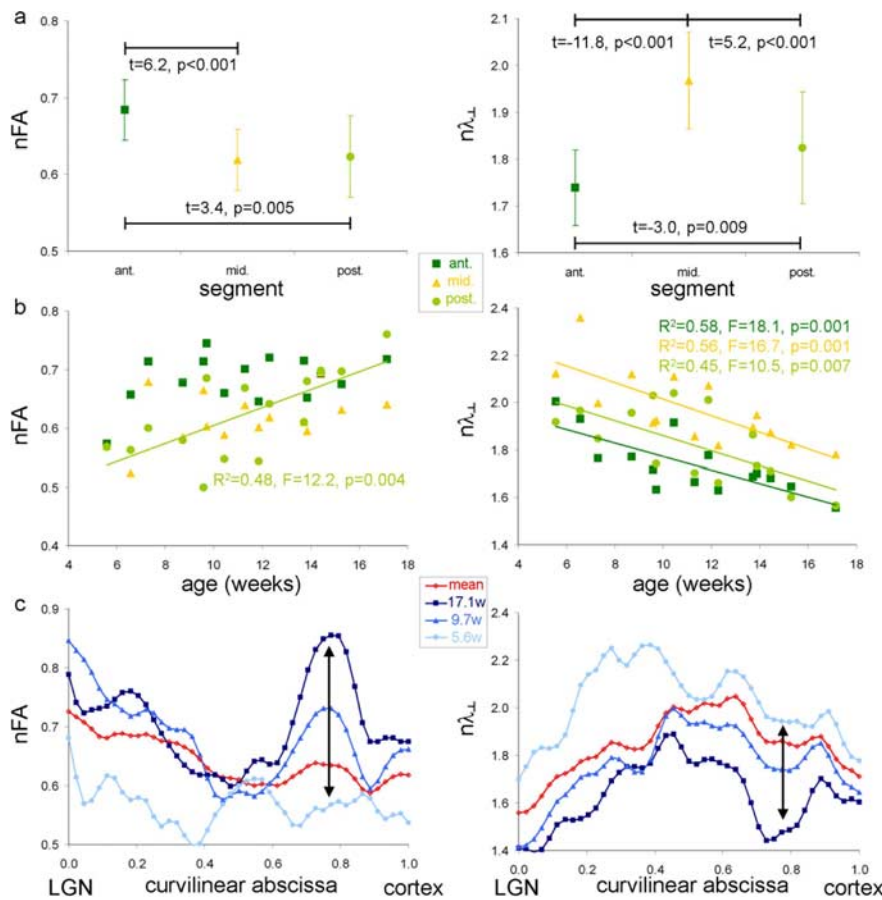
Figure 3. Heterogeneous maturation within and along the optic radiations. Left and right columns represent normalized FA and \lambda_{\perp} , respectively. a , Group mean indices, with quantification on average over the three segments (with SDs in plot bars). Advanced maturation was observed in the anterior segment, with indices closest to 1, followed by the posterior segment, with lower n\lambda_{\perp} compared with the middle segment. ant, Anterior; mid, middle; post, posterior. b , Age-related changes of indices, showing an increase in nFA in the posterior segment and decreases in n\lambda_{\perp} in all segments. c , Quantification of normalized indices along the tracts, from the LGN (abscissa, 0) to the occipital pole (abscissa, 1): mean over the infant group and results for subjects of different ages (5.6, 9.7, and 17.1 weeks of age). The topographical patterns were relatively similar across infants (normalized indices approach 1 with age and maturation), except at the level of the posterior segment where the interindividual variability was high (arrows), with a strong increase of nFA and decrease of n\lambda_{\perp} with age.
