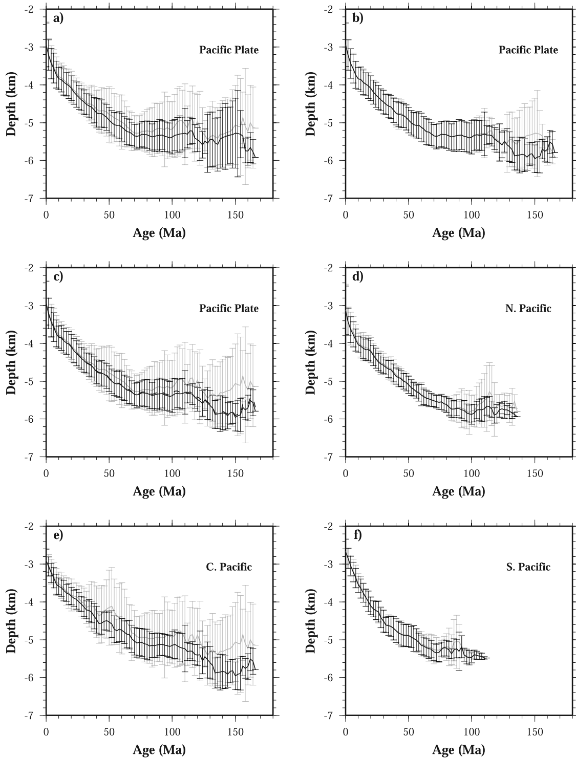
Figure 4. Mean depths and standard deviations in 2 Ma age bins versus seafloor age for the entire Pacific plate (a) before (thin lines) and after (solid lines) removal of seamounts only, (b) before (thin lines) and after (solid lines) further removal of LIPs, and (c) before (thin lines) and after (solid lines) removal of seamounts and LIPs and for different R_s = 2 (dashed line), and for (d) the northern Pacific region, (e) the central Pacific region, and (f) the southern Pacific region for the topography before (thin lines) and after (solid lines) removal of seamounts and LIPs. R_s = 3 for all except for the dashed line in Figure 4c.
