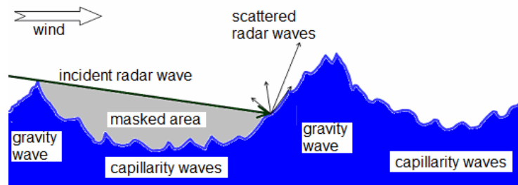
Figure 1. The phenomenological model of sea surface and interaction with electromagnetic waves
