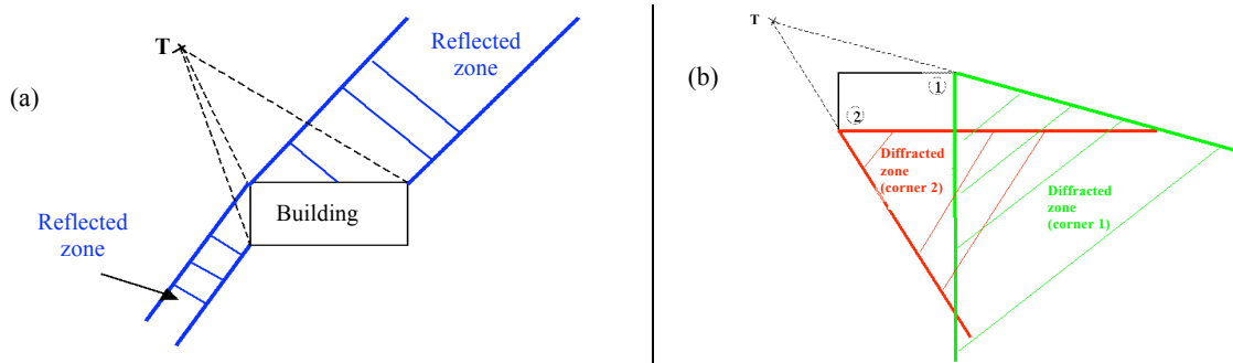
Figure 2: 2DH module : (a) – Reflected zones due to a building ; (b) – Diffracted zones due to a building
