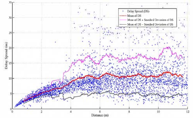
Figure 4. Delay spread dependency on Tx-Rx distance
