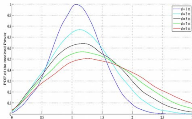
Figure 6. PDF of the received Power for various distances
