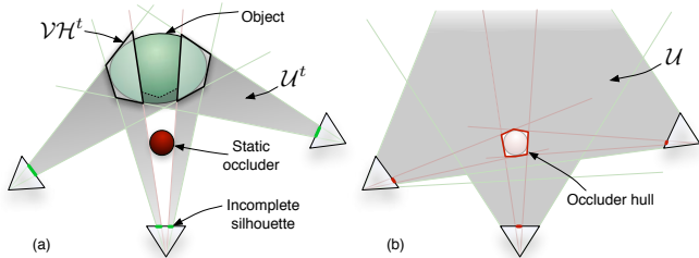
Figure 2. Deterministic occlusion reasoning. (a) An occluder-free region \mathcal{U}^t can be deduced from the incomplete visual hull \mathcal{V}\mathcal{H}^t at time t . (b) \mathcal{U} : occluder-free regions accumulated over time.
