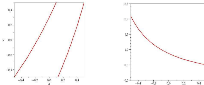
FIGURE 1. The functions T_r (left), and u_r (right), for r = -\frac{1}{2} .
