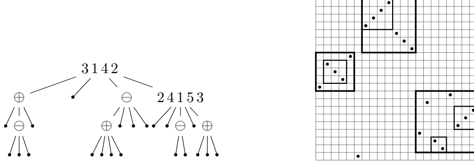
Figure 2 The substitution decomposition tree and the graphical representation (with non-trivial strong intervals marked by rectangles) of permutation \sigma = 10\ 13\ 12\ 11\ 14\ 1\ 18\ 19\ 20\ 21\ 17\ 16\ 15\ 4\ 8\ 3\ 2\ 9\ 5\ 6\ 7 .
