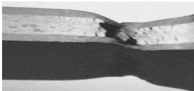
Fig. 2 Three-layered (Ti+O+Ti-alloy) composite sample tensile tested at 700°C. The test was interrupted before failure.
