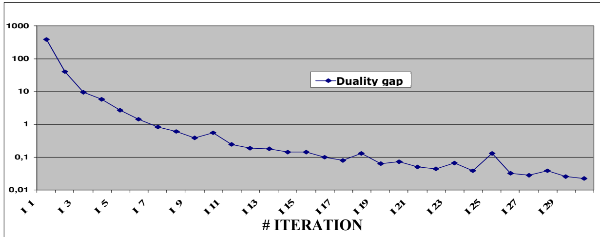
FIGURE 2 Convergence criterion against iteration number
