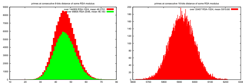
(a) Primes at consecutive 8-bit distance of some RSA modulus (b) Primes at consecutive 16-bit distance of some RSA modulus
