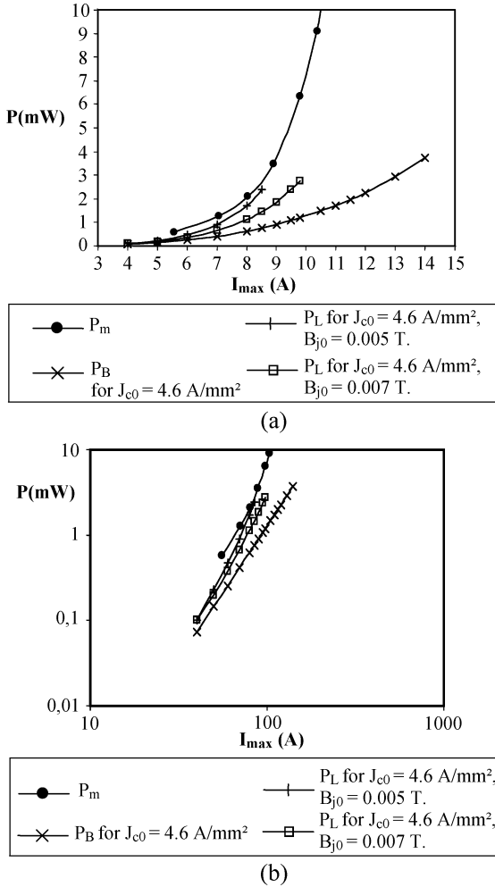
Fig. 4. Compared AC losses between the Bean model P_B , linear model P_L , and measured data P_m with (a) linear scale and (b) log-log scale.
