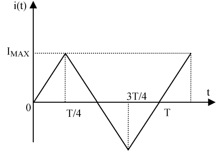
Fig. 2. Periodic current supply to the studied sample.
