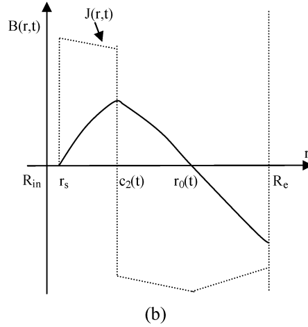
Fig. 3. Distributions of B(r, t) and J(r, t) versus r with the linear model. (a) i(t) > 0 ; (b) i(t) < 0 .
