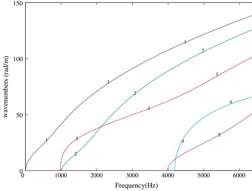
Fig. 10. WFE guided wavenumbers prediction for the rib-stiffened plate: CP boundary conditions.
