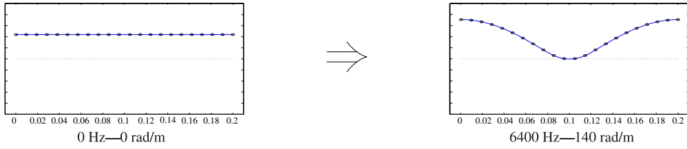
Fig. 12. Deformed shape corresponding to branch 1 at 0 Hz and 6400 Hz.
