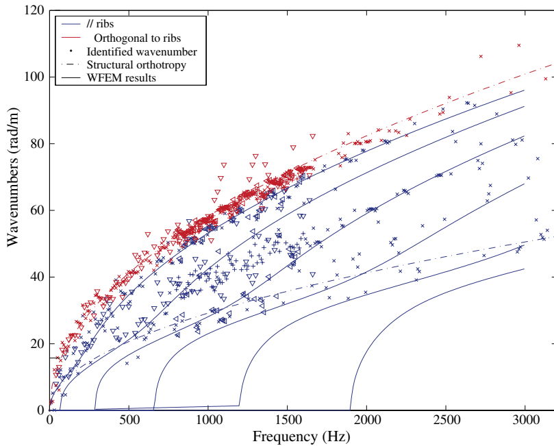
Fig. 26. Frequency dependent dominant wavenumbers for the two orthotropy direction x' and y' – case B: \star , \triangleleft experimental results.
