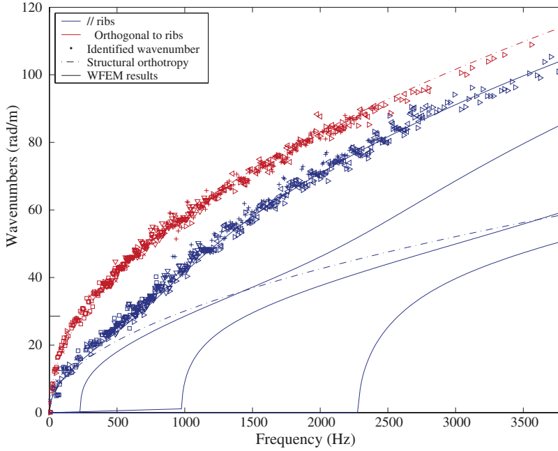
Fig. 25. Frequency dependent dominant wavenumbers for the two orthotropy direction x' and y' – case A: '+', 'o', <math>\triangleleft</math> experimental results.
