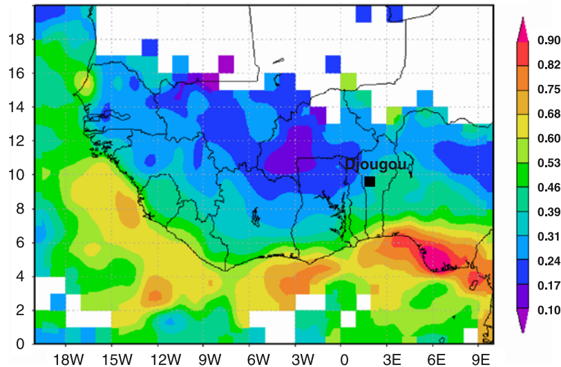
Figure 12. MODIS average AOD for the period from 18 to 24 January showing maximal values over the ocean.
