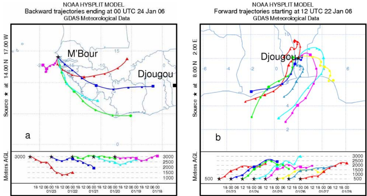
Figure 11. (a) Backward trajectories ending at M'Bour (14°N, 17°W) at 3000 m from 20 to 23 January; (b) forward trajectories of biomass burning particles emitted at 8°N, 2°E at 500 m altitude, for the period from 22 to 28 January.
