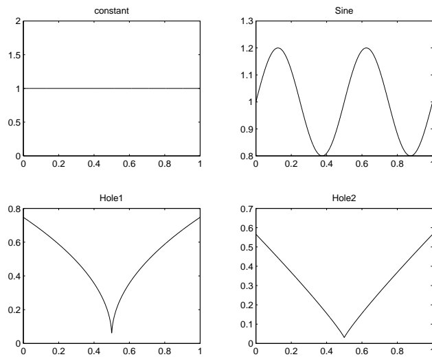
Fig. 2 Design density
