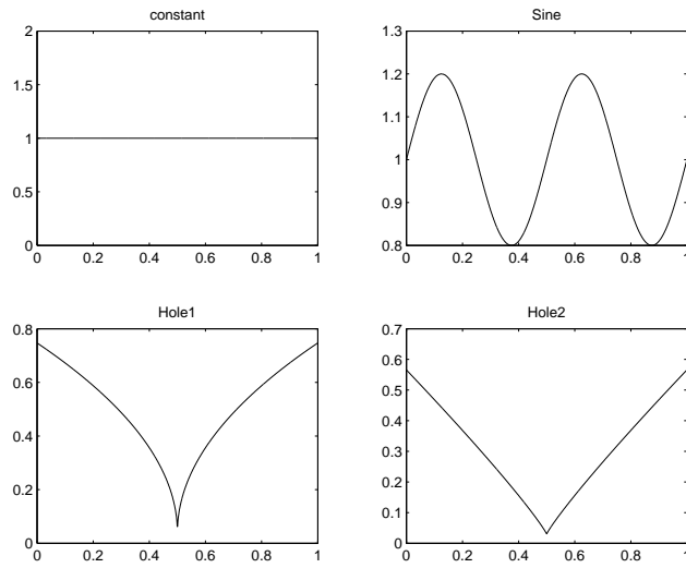
Fig. 2 Design density
