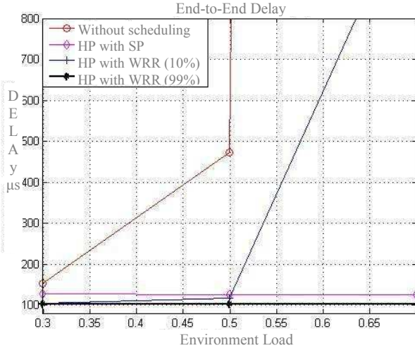
Fig. 4. Simulation results of CPN model of Ethernet switch according the scheduling policies and load environment
