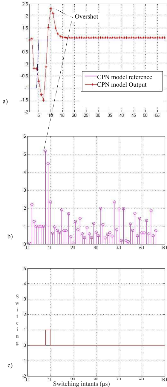
Fig. 7. Output a), delay (μs) (b) and switching instants (c) of HTCPN model and Matlab model, at 0.7 environment load.
