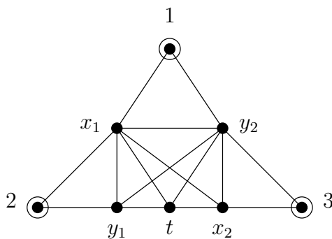
Figure 4: Graph containing a strong asteroidal triple
