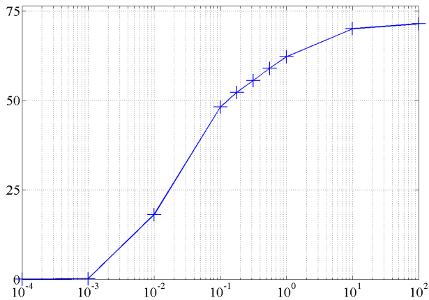
Figure 2: Percentage of coefficients set to zero as a function of the penalty factor \lambda (log scale).
