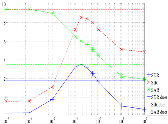
Figure 1: SDR, SIR, SAR of the proposed iterative algorithm and DUET as a function of the penalty factor \lambda (log scale).
