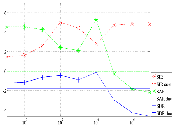
Figure 3: SDR, SIR, SAR of the proposed iterative algorithm and DUET as a function of the penalty factor \lambda (log scale).
