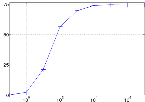
Figure 4: Percentage of coefficients set to zero as a function of the penalty factor \lambda (log scale).
