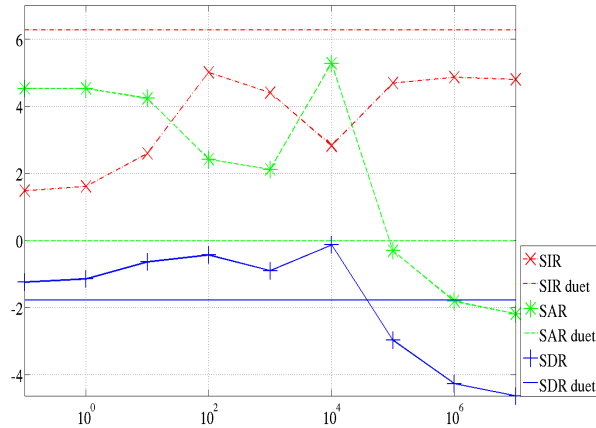
Figure 3: SDR, SIR, SAR of the proposed iterative algorithm and DUET as function of the penalty factor \lambda (log scale).
