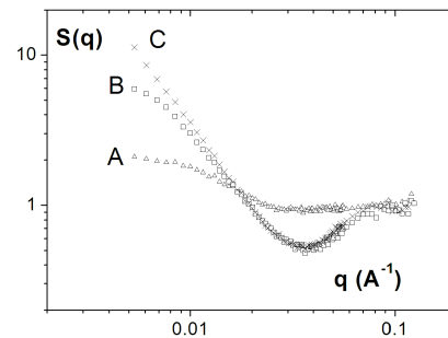
Fig 4 – Nanoparticle structure factor of cluster dispersions based on MNP2 nanoparticles and A, B or C copolymer.
