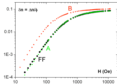
Fig6 - Static magneto-optical birefringence \Delta n normalized by the volume fraction \Phi of nanoparticles in the dispersions. Lower curves : pure ferrofluid FF and dispersion of NP2/A-copolymer clusters; upper curve dispersion of NP2/B-copolymer clusters.
