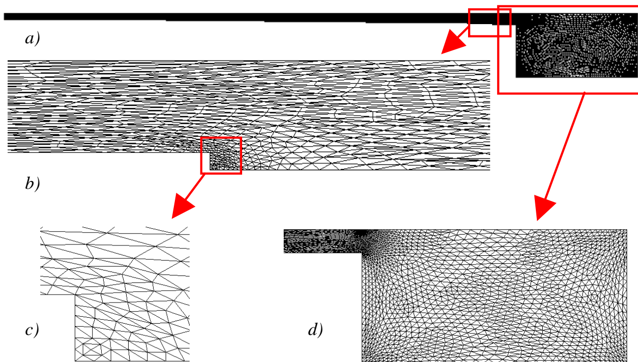
Figure 2 Optimized mesh of the back chamber after 16 mesh adapting iterations a) , detailed view near a step of the backing electrode b) c) , detailed view of the mesh in the peripheral reservoir d) .
