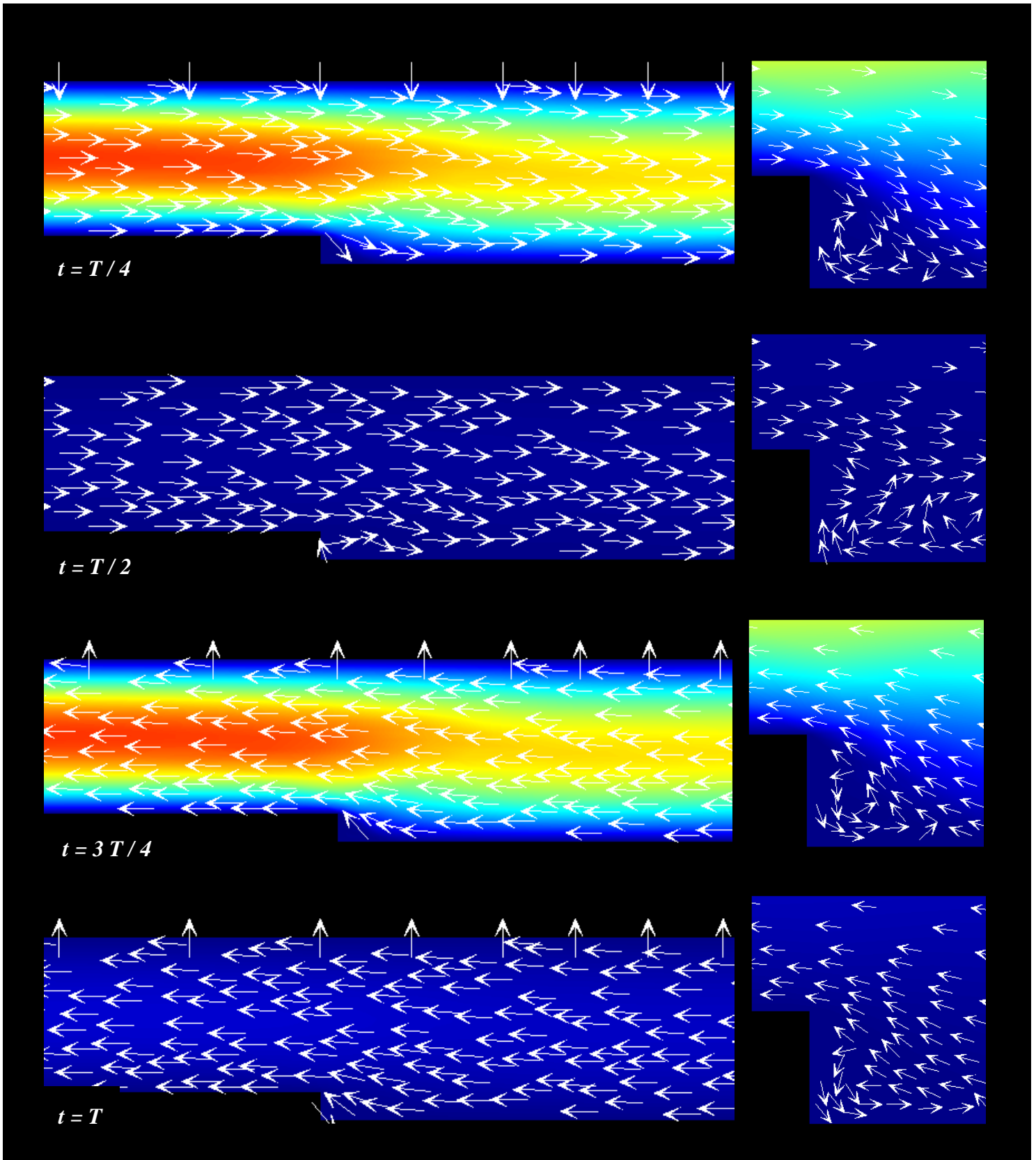
Figure 3 Particle velocity near the right step of the backing electrode.
