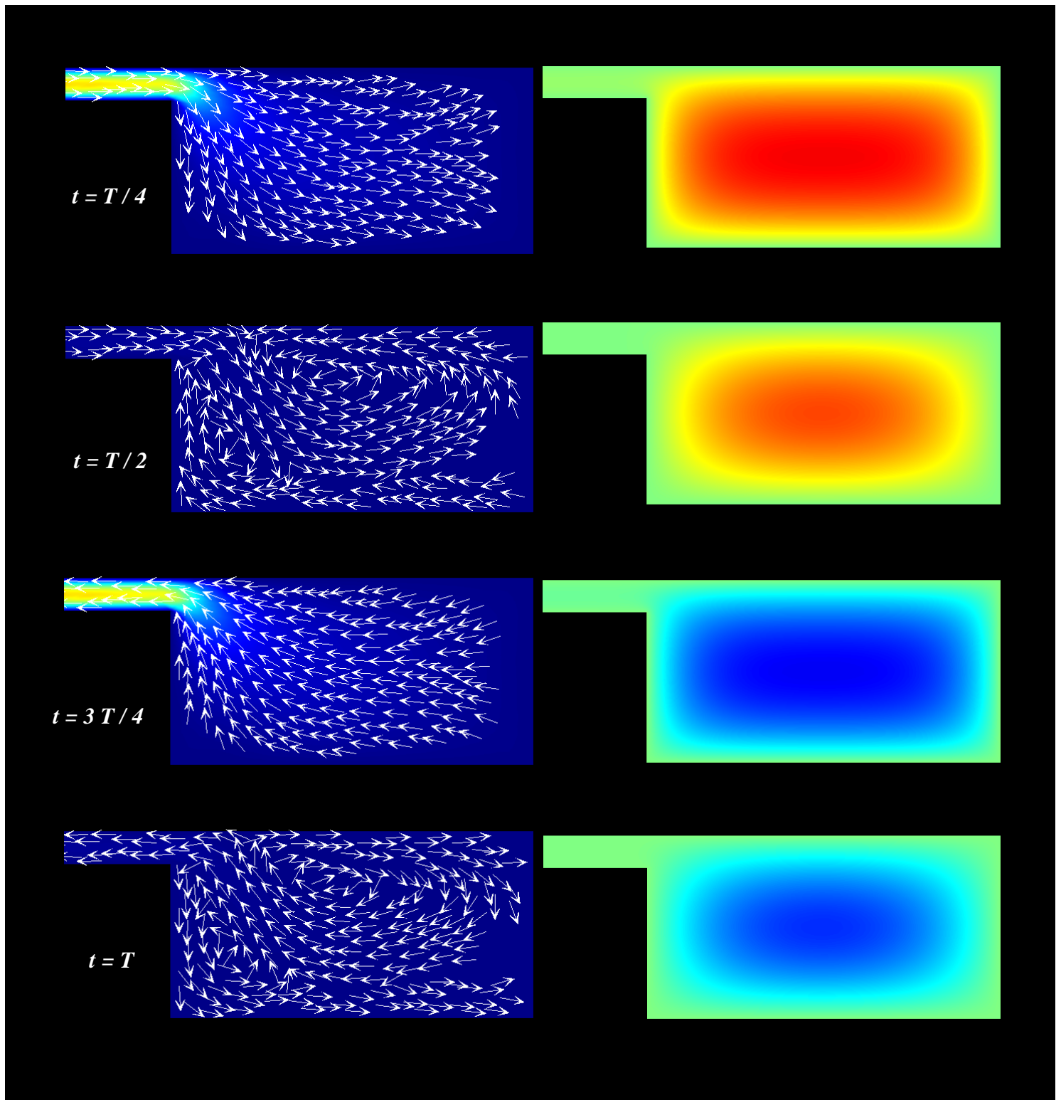
Figure 4 Particle velocity (left) and temperature variation (right) in the peripheral cavity (mesh of Fig. 2d).
