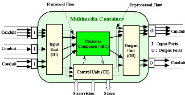
Figure 4. Internal architecture of an Elementary Processor
