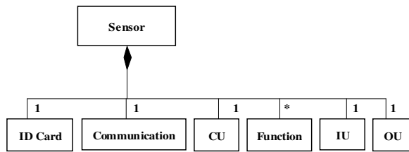
Figure 5. Class diagram of an Elementary Processor
