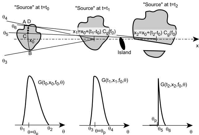
Figure 6. Dispersion of linear waves in two dimension, represented here on a flat surface for simplicity. The variable y has been dropped as the spectra shown here are all at y = 0 . We call "source" the region of the ocean where waves with frequencies smaller than f_{\min} can be found. As time goes by, the source expands in space due to both frequency dispersion (like in 1D), and geometrical dispersion. The wave energy with frequency f_0 that will be observed at point x_1 (respectively x_2 ) at time t_1 (respectively t_2 ) is, at time t_0 , along the thin arc circle AB (respectively the thick dotted arc circle CD). Due to the small island between x_1 and x_2 , the energy that would have been recorded at x_2 , if the island were not present, is actually dissipated on the shore of the island. As a result the local energy density E(x_2) is reduced. At frequency f_0 , contributions to E(x_2) only come from angles \theta_5 to \theta_6 . The directional spectra (bottom) are thus affected by the blocking effect of islands, and the directional narrowing as one goes further from x_0 (on the Earth this narrowing reverses after 10000 km of propagation, due to the sphericity).
