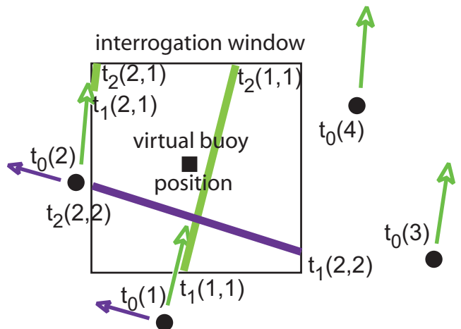
Figure 1. Schematic definition of a virtual buoy. Any SAR observation i is available at a time t_0(i) on the black dots. All swell partitions (i, j) (here indicated by the arrows) are propagated and may cross the interrogation window from time t_1(i, j) to t_2(i, j) .
