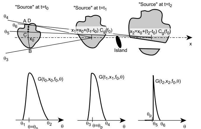
Figure 7. Dispersion of linear waves in two dimension, represented here on a flat surface for simplicity. The variable y has been dropped as the spectra shown here are all at y = 0 . We call "source" the region of the ocean where waves with frequencies smaller than f_{\min} can be found. As time goes by, the source expands in space due to both frequency dispersion (like in 1D), and geometrical dispersion. The wave energy with frequency f_0 that will be observed at point x_1 (respectively x_2 ) at time t_1 (respectively t_2 ) is, at time t_0 , along the thin arc circle AB (respectively the thick dotted arc circle CD). Due to the small island between x_1 and x_2 , the energy that would have been recorded at x_2 , if the island were not present, is actually dissipated on the shore of the island. As a result the local energy density E(x_2) is reduced. At frequency f_0 , contributions to E(x_2) only come from angles \theta_5 to \theta_6 . The directional spectra (bottom) are thus affected by the blocking effect of islands, and the directional narrowing as one goes further from x_0 (on the Earth this narrowing reverses after 10000 km of propagation, due to the sphericity).
