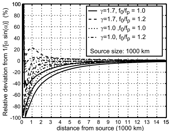
Figure 11. Convergence of the swell energy E_s integral (C1) towards the asymptote 1/(\alpha \sin \alpha) , as a function of spectrum width for a storm diameter of 1000 km. The result is independent of the choice of f_p . In practice the calculations were made for f_p = 0.07 Hz ( T_p = 13 s). The three lines for each case correspond to position errors \Delta_x of -200, 0 and 200 km relative to the great circle trajectory. For all cases considered here the deviation is less than 20% beyond 4000 km from the storm center.
