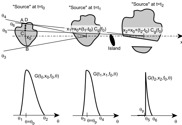
Figure 6. Dispersion of linear waves in two dimension, represented here on a flat surface for simplicity. The variable y has been dropped as the spectra shown here are all at y = 0 . We call "source" the region of the ocean where waves with frequencies smaller than f_{\min} can be found. As time goes by, the source expands in space due to both frequency dispersion (like in 1D), and geometrical dispersion. The wave energy with frequency f_0 that will be observed at point x_1 (respectively x_2 ) at time t_1 (respectively t_2 ) is, at time t_0 , along the thin arc circle AB (respectively the thick dotted arc circle CD). Due to the small island between x_1 and x_2 , the energy that would have been recorded at x_2 , if the island were not present, is actually dissipated on the shore of the island. As a result the local energy density E(x_2) is reduced. At frequency f_0 , contributions to E(x_2) only come from angles \theta_5 to \theta_6 . The directional spectra (bottom) are thus affected by the blocking effect of islands, and the directional narrowing as one goes further from x_0 (on the Earth this narrowing reverses after 10000 km of propagation, due to the sphericity).
