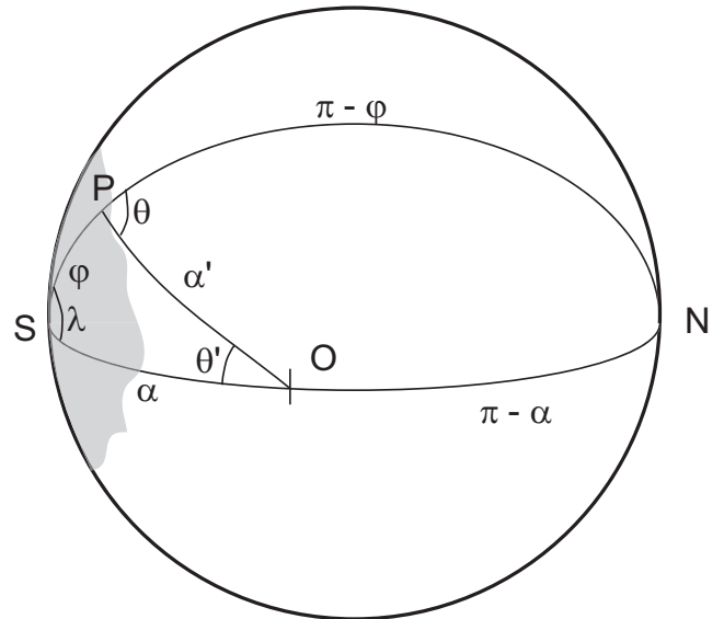
Figure 7. Geometry of the "fossil" swell field distribution at time t_0 = 0 (shaded area) and observation conditions. Any point P of colatitude \varphi and longitude \lambda inside of the storm, generates waves that are observed at point O . At time t the observed waves that come from P have a well defined frequency given by eq. (C2), function of the spherical distance \alpha' between P and O , and a well defined direction \theta at P , relative to the North, which gives a direction \pi - \theta' at O . In the triangle OPS the angles \lambda , \theta' and \pi - \theta are related to the distances \alpha' , \varphi and \alpha by the usual spherical trigonometry relationships, e.g. eq. (C4).
