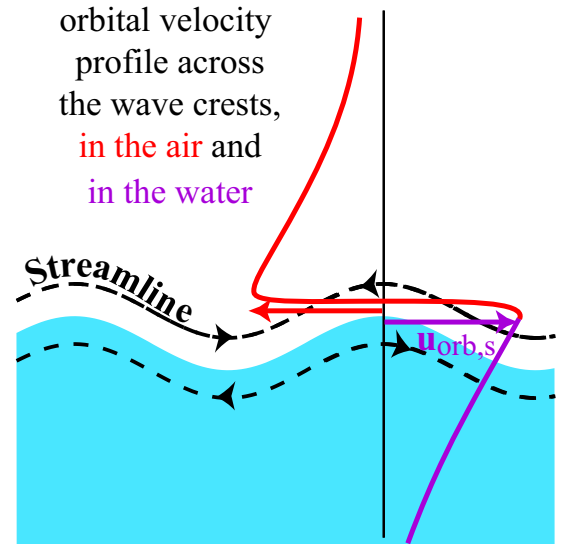
Figure 9. Boundary layer over waves in the absence of wind. Because of the larger inertia of the water compared to the air, most of the adjustment from the sub-surface velocity to the free stream velocity in the air occurs on the air-side of the surface.
