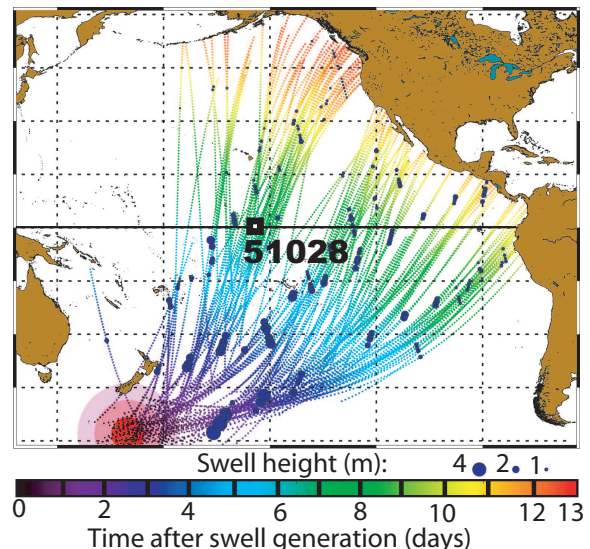
Figure 4. Finding the source storm. All swells with a 17 \pm 0.5 s period that were identified in 13 days of ENVISAT synthetic aperture radar data over the Pacific, are re-focused from their location of observation (filled dots) following their direction of arrival at the theoretical group speed for 17 s waves. This focussing reveals a single swell generation event, well defined in space and time (pink to red disks). The back-tracking trajectories are color-dated from black (July 9 2004 18:00 UTC) to red (July 22 2004 18:00 UTC).
