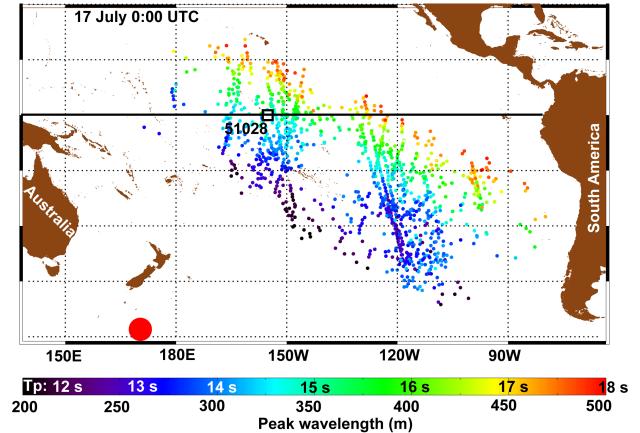
Figure 3. Snapshot of the “fireworks” animation given in the auxiliary material, for July 17 2004 at 0:00 UTC. Each of the 1071 colored dots represent one observed swell partition, within 6 days of its observation, displaced along a great circle with the group speed corresponding to the detected peak period in the direction of the detected peak direction. Only swells with tracks that passes within 1000 km of the storm center (red disk) have been retained.
