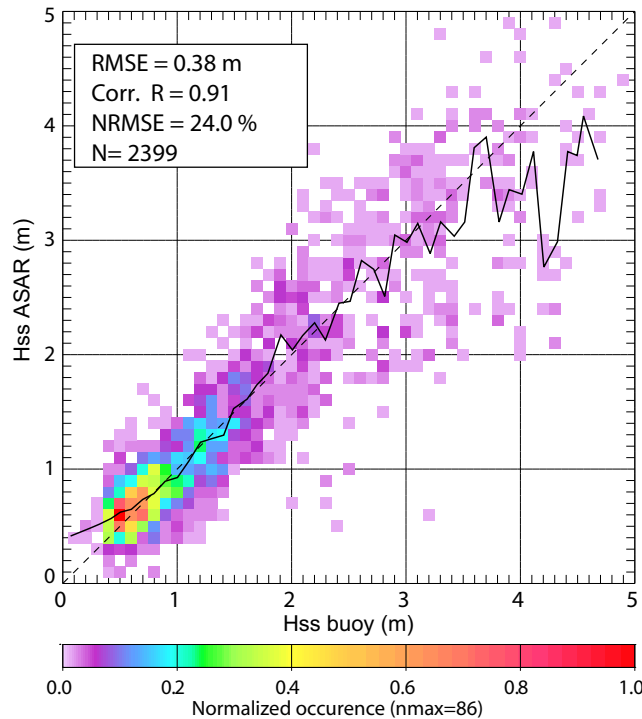
Figure 10. ASAR-derived swell partition heights versus buoy swell partition heights after bias correction using eq. (3), for subset A. The solid line joins the median values from SAR observations in each 0.1 m class of buoy-measured height.
