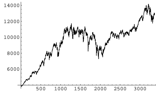
Figure 6. The Dow Jones 30 Industrials from 03.01.1995 to 30.05.2008.
