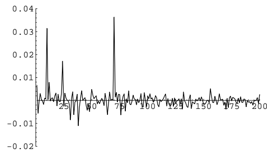
Figure 5. Ramanujan-Fourier transform of a period modulated cosine function: n_0 = 10 and n_1 = 14 .
