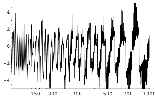
Figure 7. The Ramanujan sums analysis of the Dow Jones 30 Industrials. Periods in the range n = 100 to n = 1000 were selected. One clearly sees (positive and negative) peaks centered about non-equally-spaced periods.
