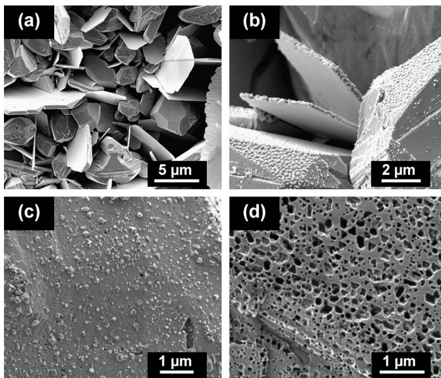
Fig. 5. SEM images of silver deposits by galvanostatic means onto smooth nickel (electricity amount: 0.3 \text{ C cm}^{-2} , image A) and glassy carbon (electricity amount: 0.6 \text{ C cm}^{-2} , image C), where the silver deposit was transformed into an Ag–Pd layer. These two kinds of surface were used as catalysts for the reductive coupling of RBr in different solvents containing 0.1 \text{ M TBABF}_4 at -1.3 \text{ V} vs. SCE. Reduction of 1-bromodecane in PC at Ni–Ag (image B) and 1-bromooctane in DMF at Ag–Pd supported by glassy carbon (image D). The electricity amounts were 0.6 \text{ C cm}^{-2} in both experiments.
