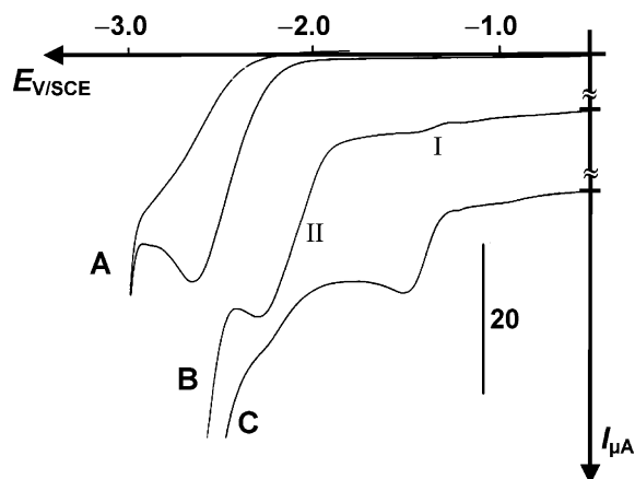
Fig. 1. Voltammograms obtained at different working electrodes using 1-bromooctane (concentration: 10 mM) in 0.1 M TBAPF 6 /DMF. Apparent surface areas, S = 0.78 \text{ mm}^2 . Scan rate: 100 \text{ mV s}^{-1} : (A) Glassy carbon, (B) Smooth silver with the separation of two steps: I and II, (C) Ag-Pd electrode.
