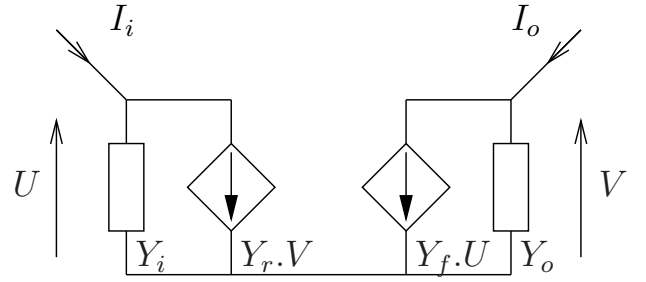
Figure 8: Reduced form of the amplifier.
