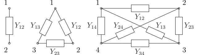
Figure 4: Representation of some n -terminal networks.
